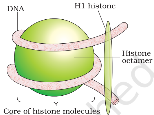
Figure 6.4a Nucleosome
