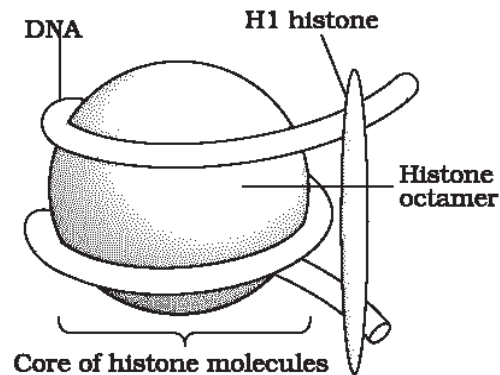
Figure 6.4a Nucleosome
