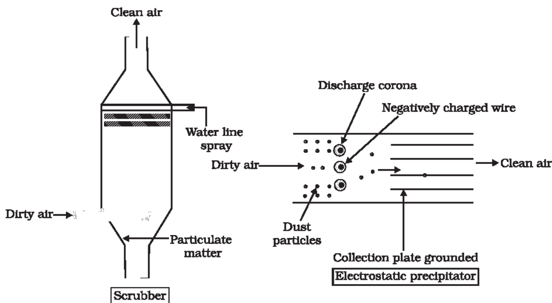
Figure 16.1 Electrostatic precipitator
